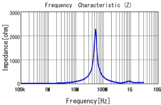
■ FDSD0630-H-1R5N |Z|
