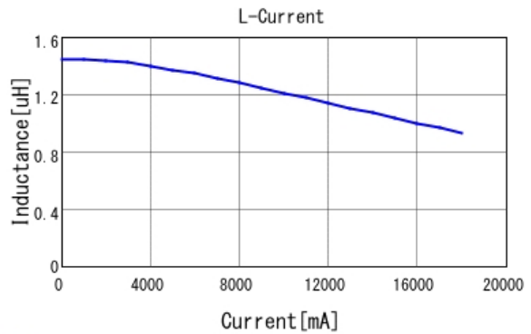
■ FDSD0630-H-1R5N L-Current 20degC
