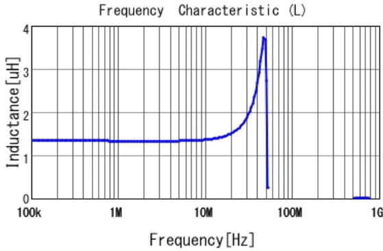
■ FDSD0630-H-1R5N L
