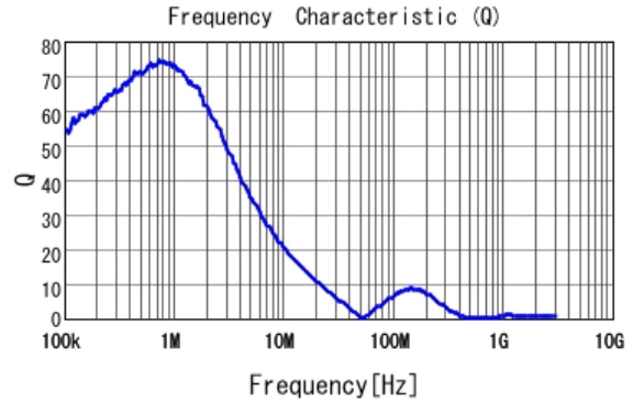
■ FDSD0630-H-1R5N Q
